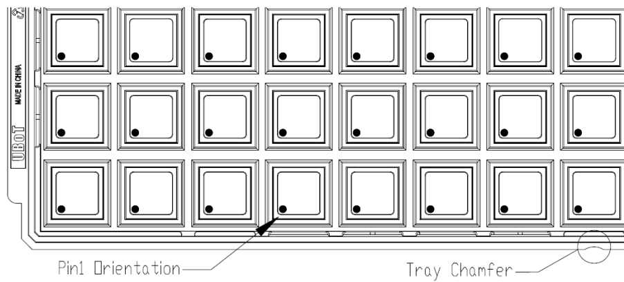
Figure 20 Tray Packaging Schematic Diagram
