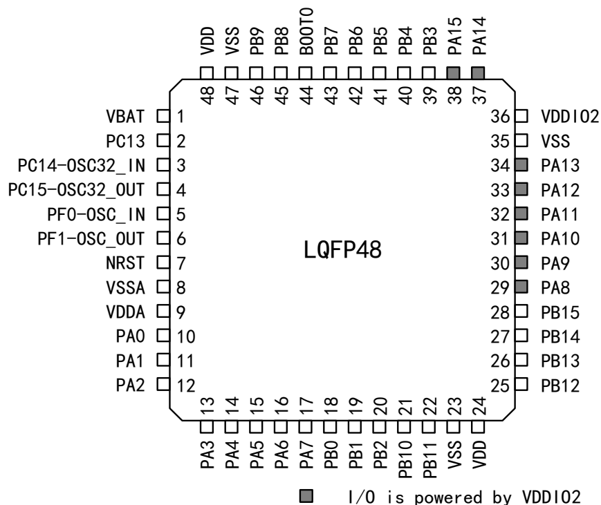
Figure 1 Pin Distribution Diagram of APM32A072xBTx Series LQFP48
