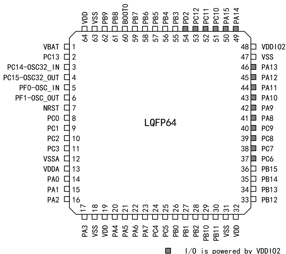
Figure 2 Pin Distribution Diagram of APM32A072xBTx Series LQFP64
