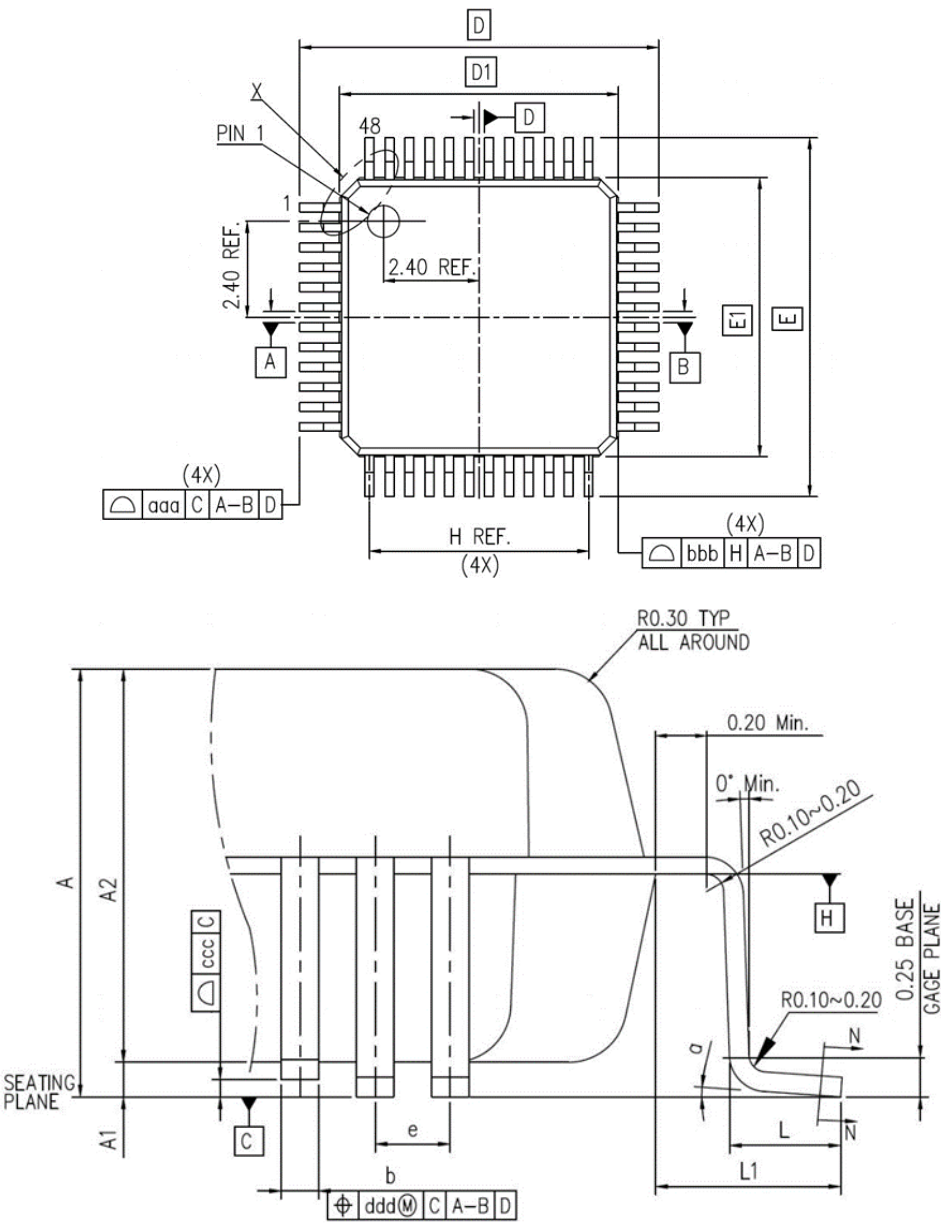
Figure 14 LQFP48 Package Diagram
