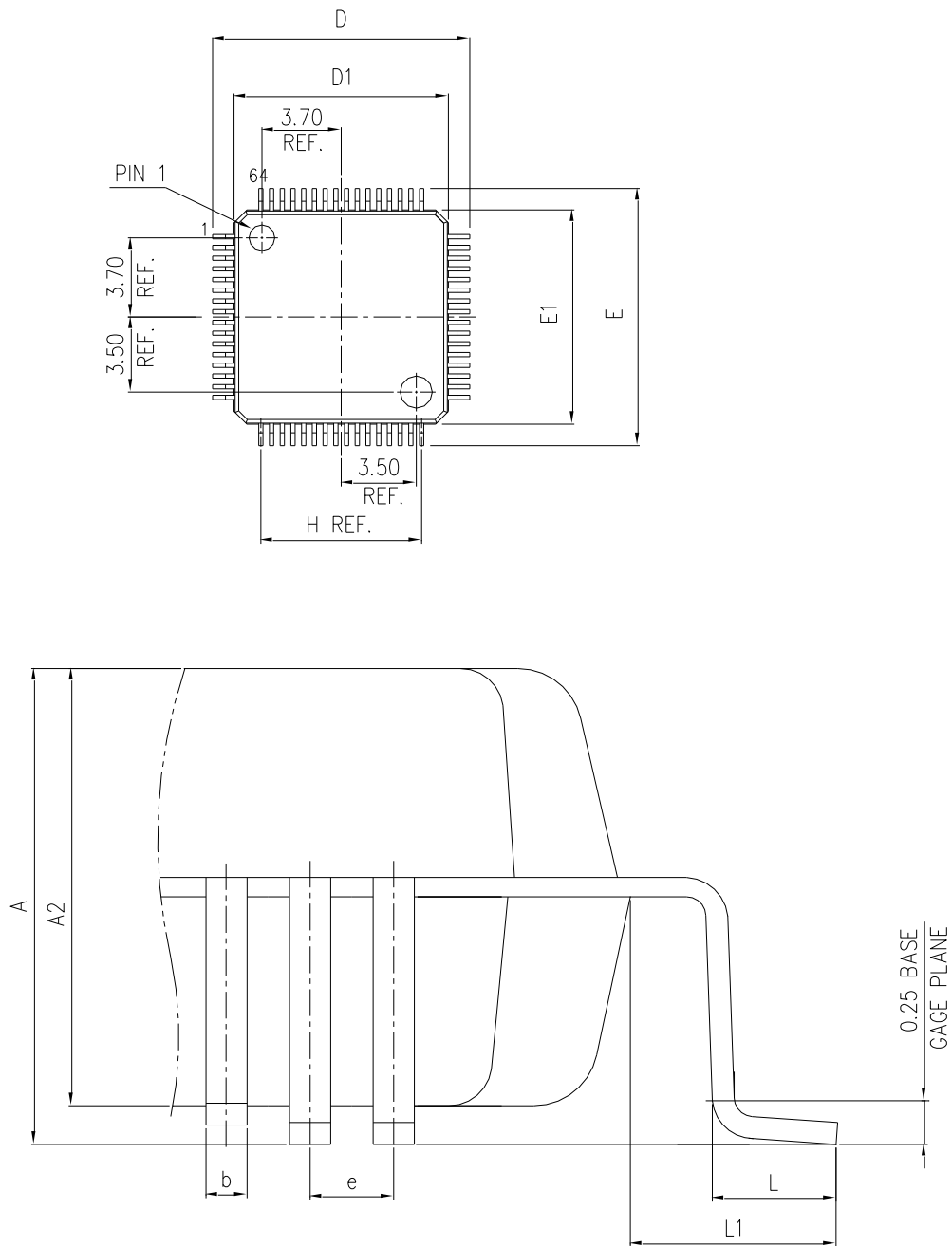
Figure 16 LQFP64 Package Diagram
