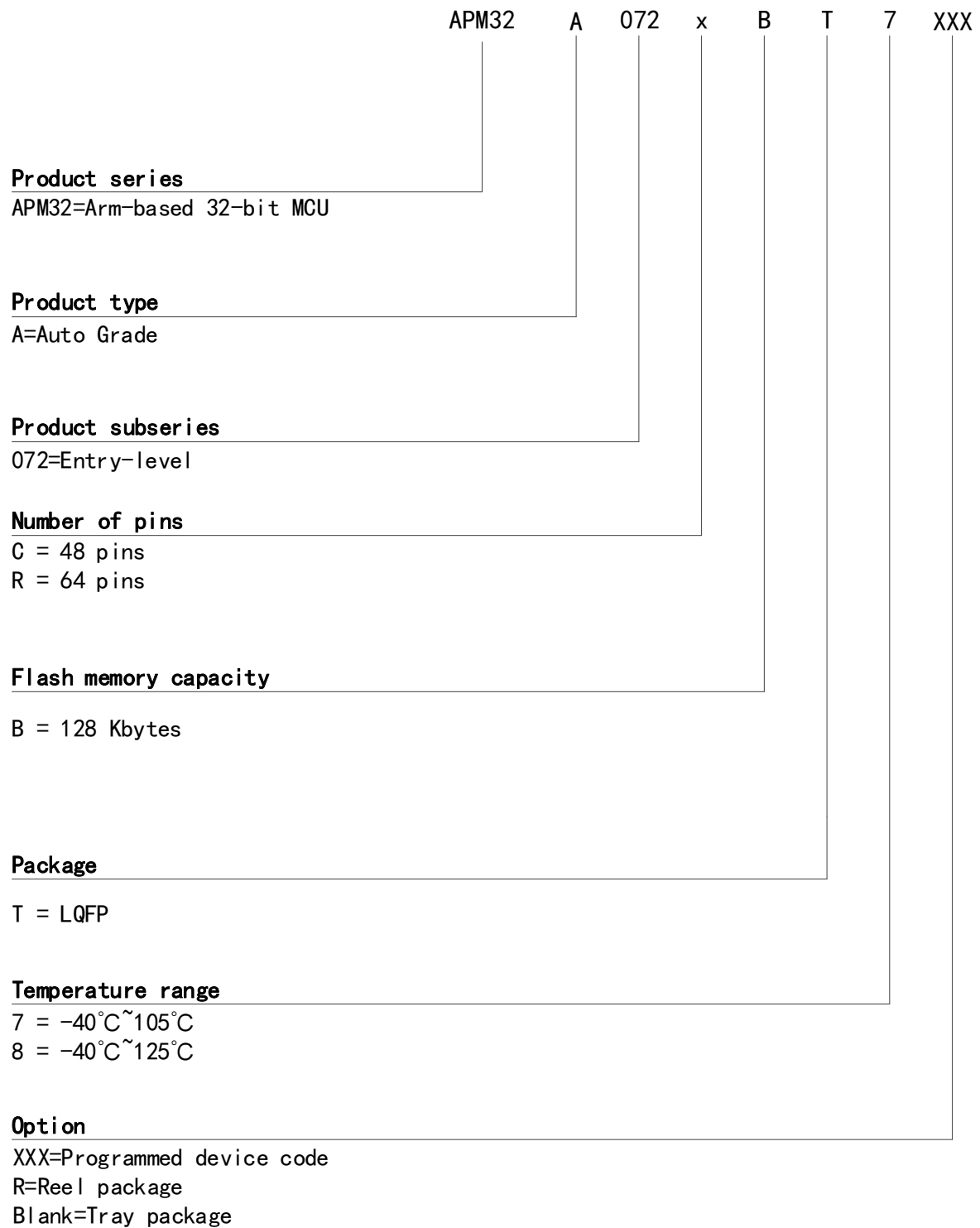
Figure 21 Naming Rules of Ordering Information
